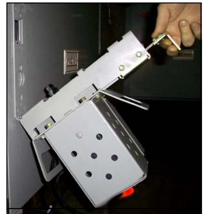
Easy mount motor operator on mounting bracket.
